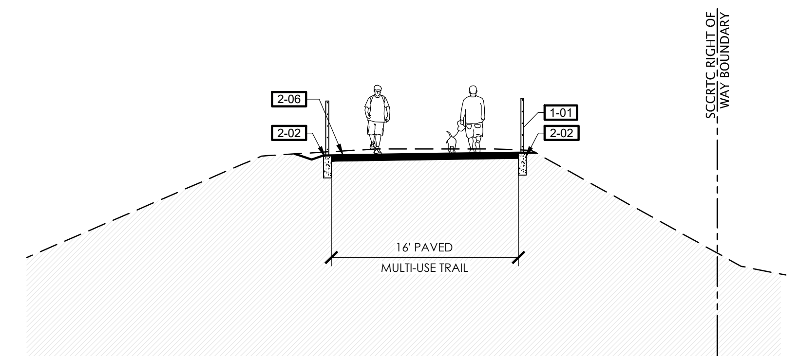
6 TYPICAL SECTION SCALE 1/8"=1'-0"
