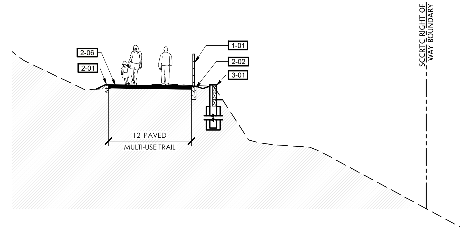
4 TYPICAL SECTION SCALE 1/8"=1'-0"
