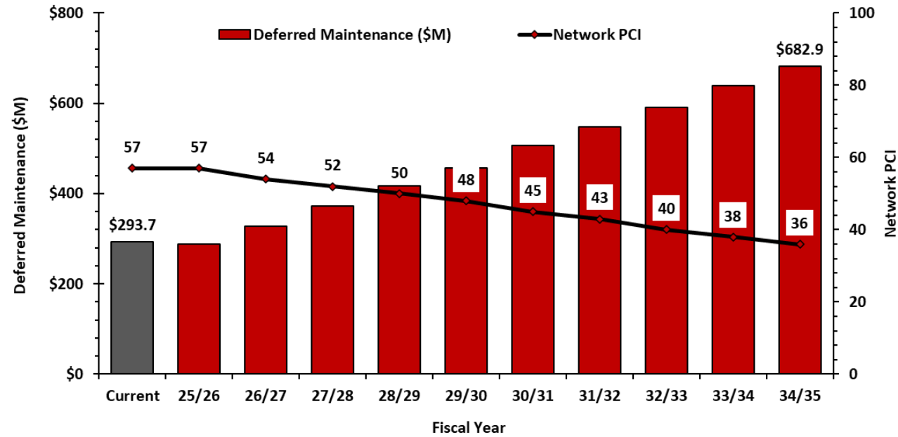
Figure 8. PCI versus Deferred Maintenance for Scenario 1.
