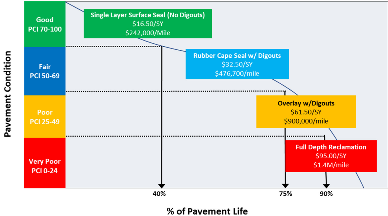
Figure 7. Costs 6 of Maintaining Arterial over Service Life.
